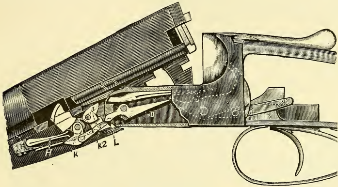
Maleham's Ejector Gun.
